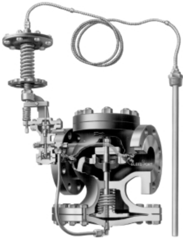
TYPE ET124 TEMPERATURE & PRESSURE REGULATOR
